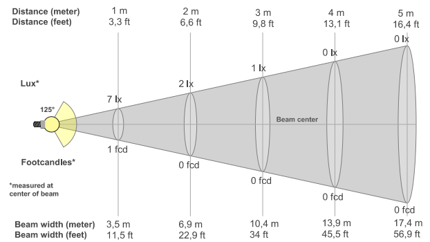
Beam details
